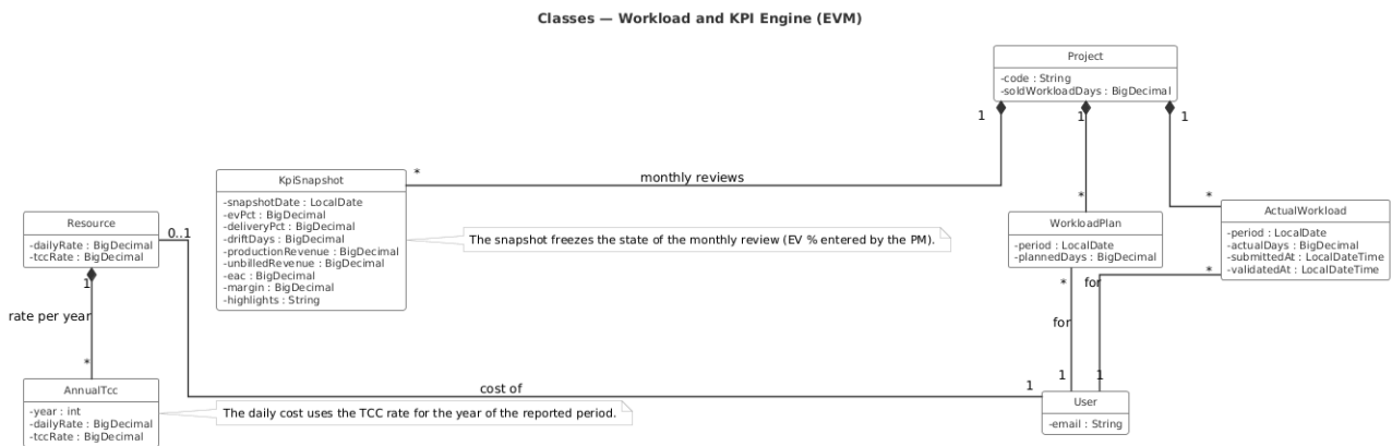
Figure 6.9: Class diagram — workload and indicator engine
